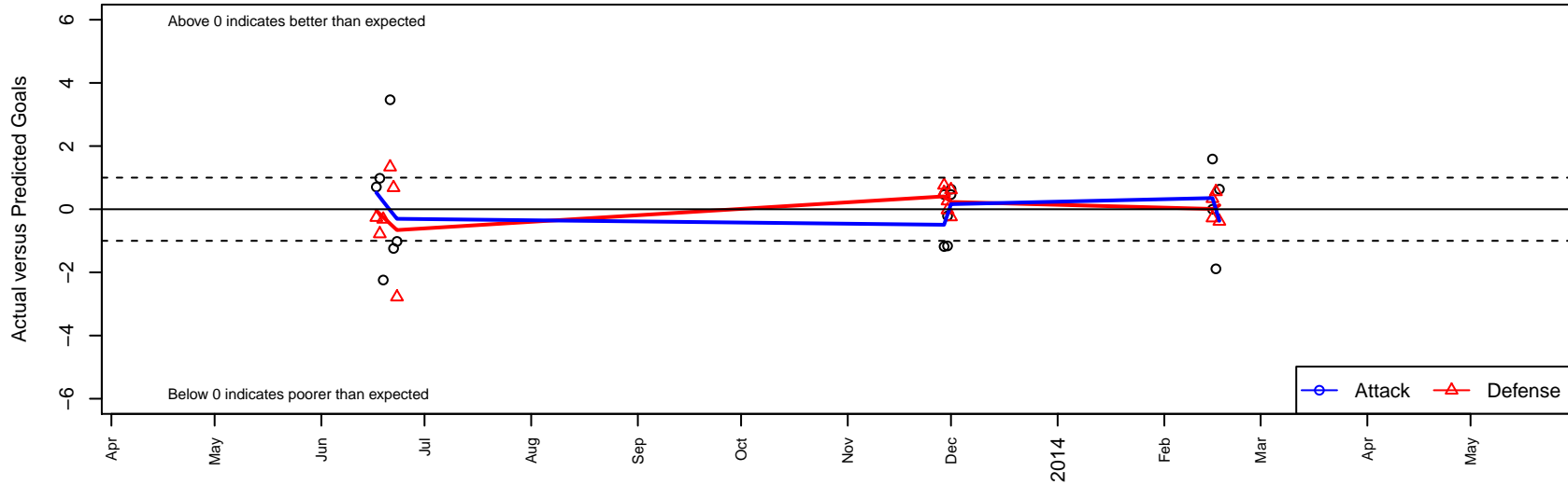
SC del Sol Leebrook White B99 Dots are actual minus expected GF (blue circles) and GA (red triangles). Blue line is smoothed change in attack strength. Red is smoothed change in defense strength.
